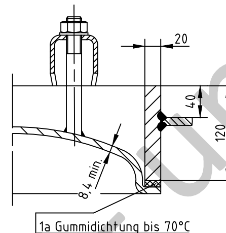
Detail X
